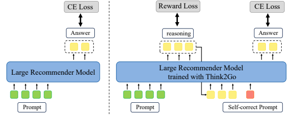
Figure 1: The architecture overview of Think2Go, which unifies RL-based reasoning and SFT within the auto-regressive generation process, connecting reasoning and supervised answers through self-correction.
