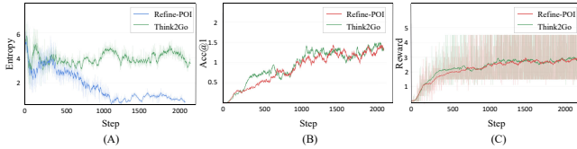
Figure 3: Advantage Estimation Analysis. We compare Refine-POI, which uses the standard GRPO method, with Think2Go, and analyze the training dynamics of Entropy, Acc@1, and Reward under each approach.
